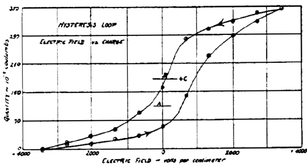
Fig. 8: The first published hysteresis curve [9]
