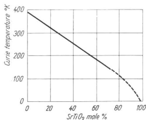
Fig. 12: Temperature of phase transition in solid solution of (\text{Ba,Sr})\text{TiO}_3 vs. composition [21]
